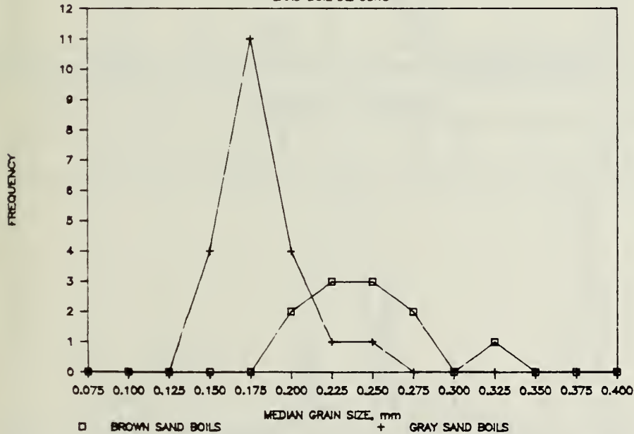
Figure 2A. Grain size frequency of subsurface units. In 2A the peak at 0.200 mm indicates that 6 samples have median grain sizes between 0.175 mm and 0.200 mm. The median grain sizes of the different subsurface units generally do not overlap. 2B. Grain size frequency of sand boils. Gray sand boils have a finer median grain size than the brown sand boils.
